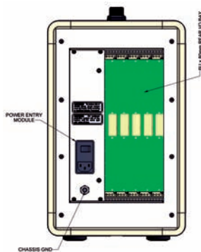
Series 815 full 6U x 80MM plug-in rear I/O
