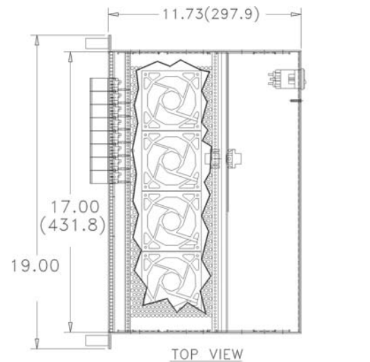
Backplane Standard Series 2345 shown with single power supply. Versions with ATX or DC power supply available. cPCI, PXI or VMEJ1 (See Pages 18, 19, 21)
